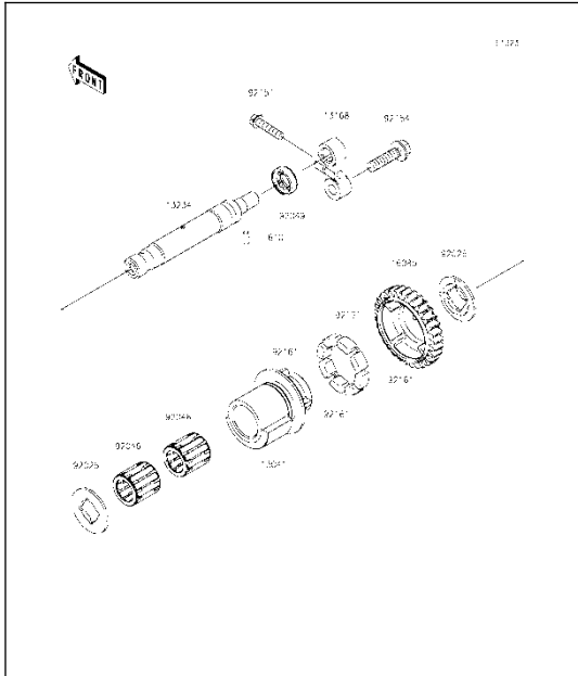
K9 Balancer
