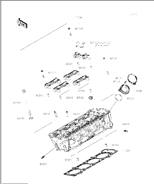
K1 Cylinder Head
