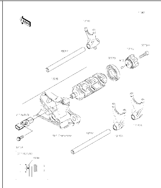
K12 Gear Change Drum/Shift Fork(s)
