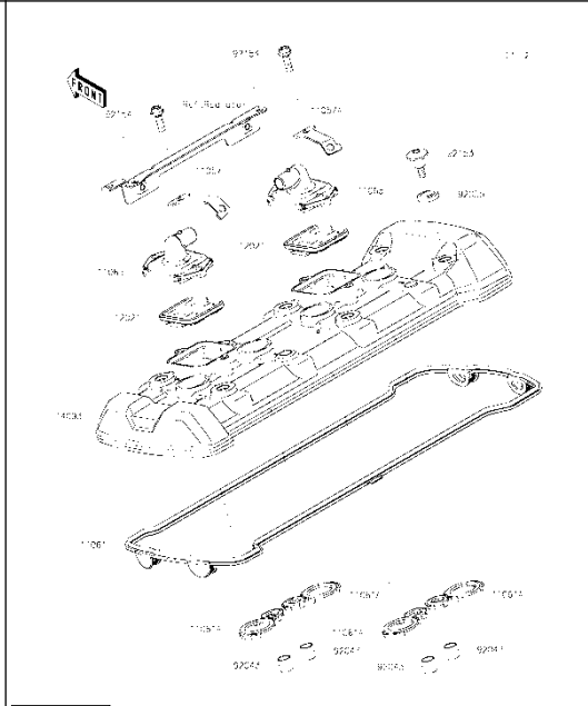
K2 Cylinder Head Cover
