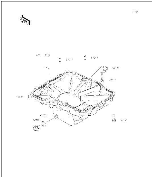
K17 Oil Pan
