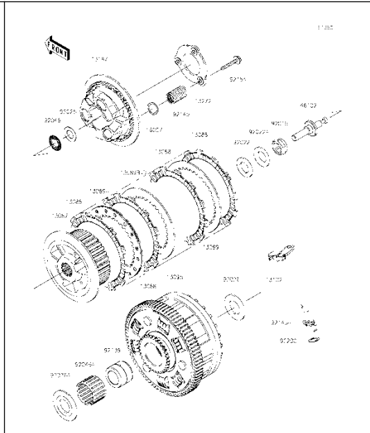
K10 Clutch
