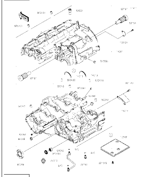
K14 Crankcase
